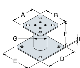
PPA100
